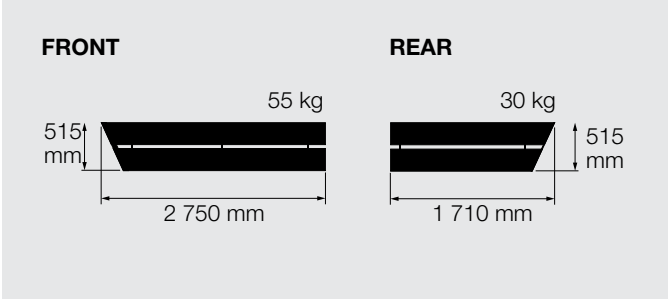
COUNTERWEIGHT
