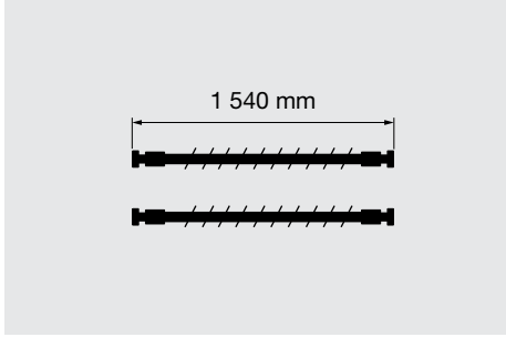
HOSE OF BOOM CYLINDERS 9 kg X 2 / 13 kg X 2
